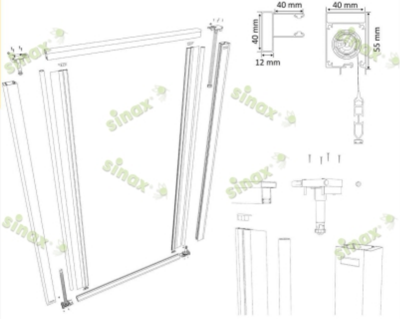
EGE 40 DOUBLE YATAY
