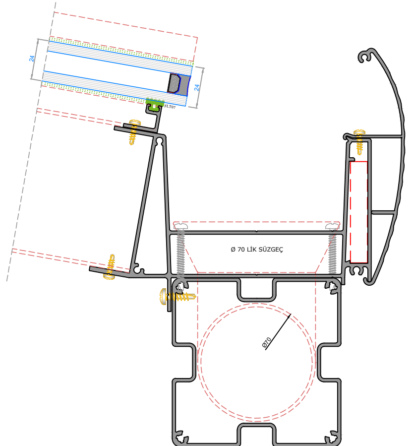
FC50-162 OLUK KAPAK GUTTER COVER
