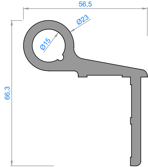
4531 - 1,690 kg/m
