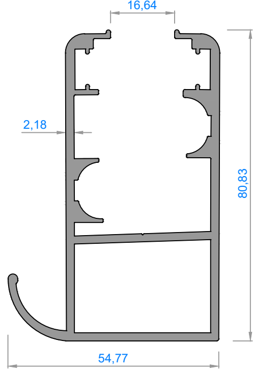
* 4354 - 1,862 kg/m
