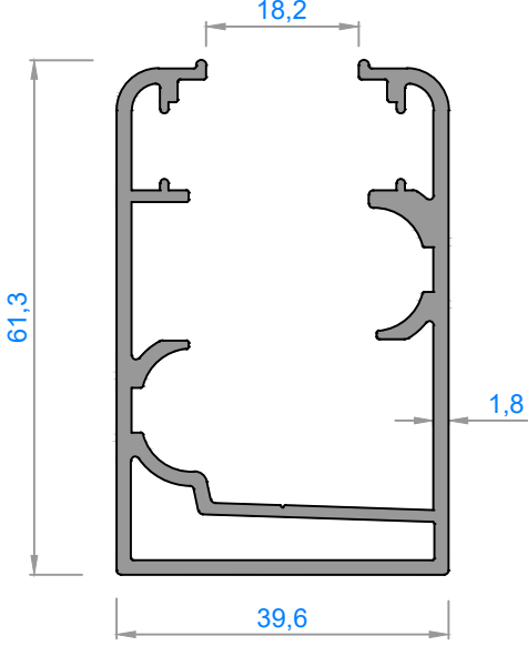
4910 - 1,210 kg/m
