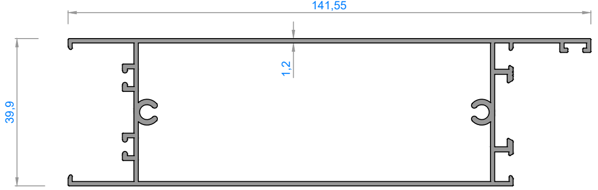
4087 - 1,343 kg/m
