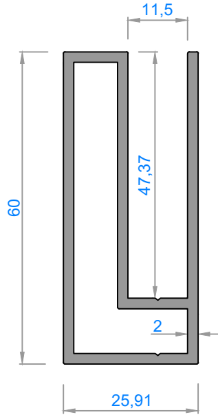
* 4011 - 1,150 kg/m
