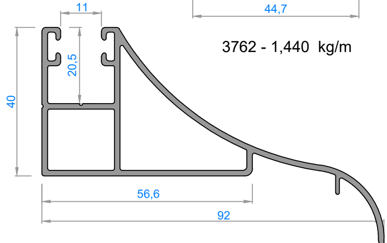
4767 - 1,112 kg/m
