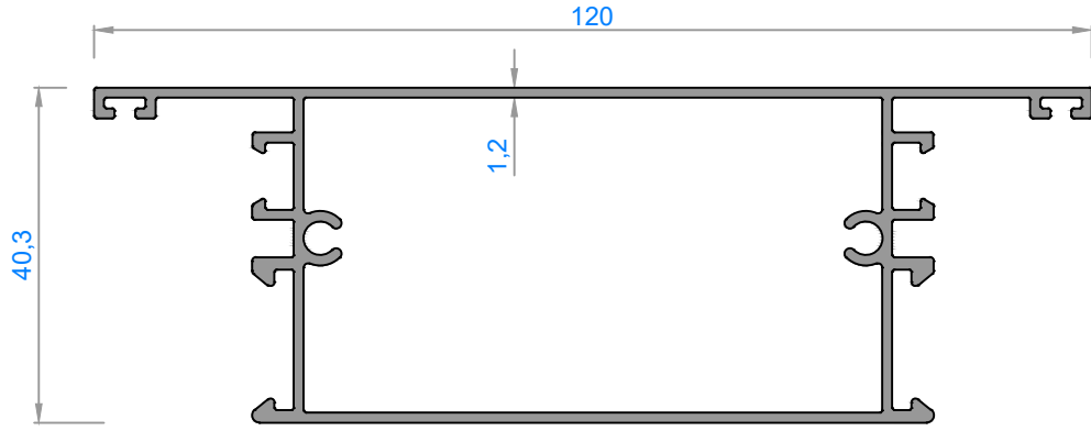
3457 - 1,184 kg/m
