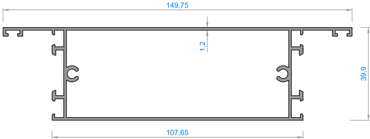
4086 - 1,351 kg/m
