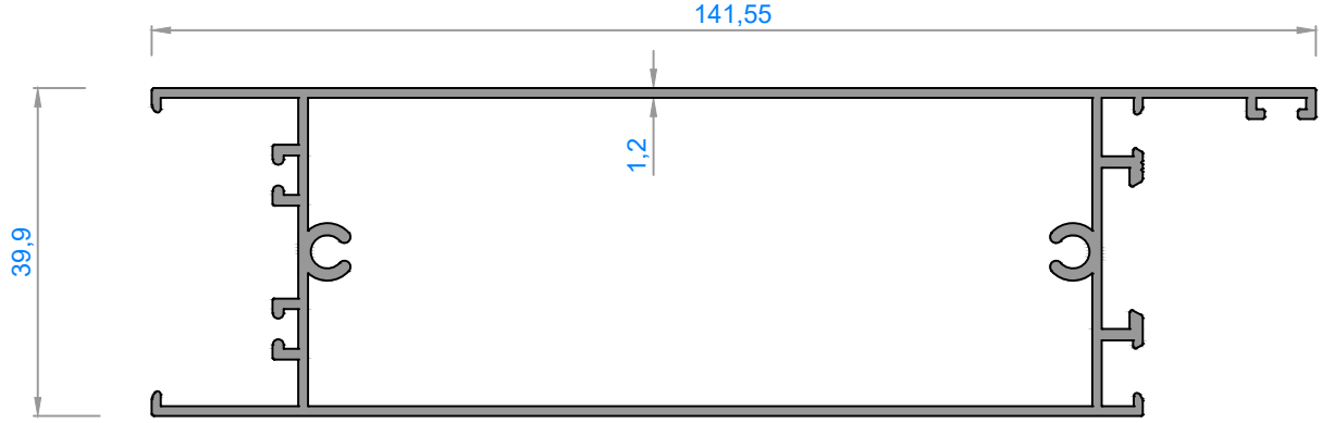
4087 - 1,343 kg/m
