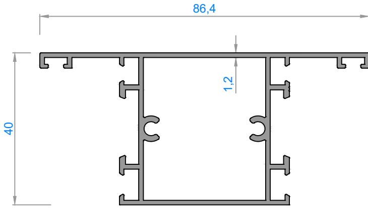
4088 - 1,032 kg/m
